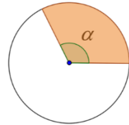
Sector circular
