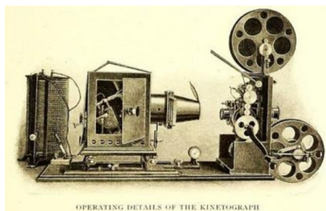
OPERATING DETAILS OF THE KINETOGRAPH
