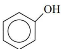
fenol
