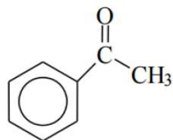
acetofenona
