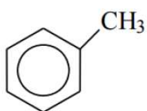
tolueno
