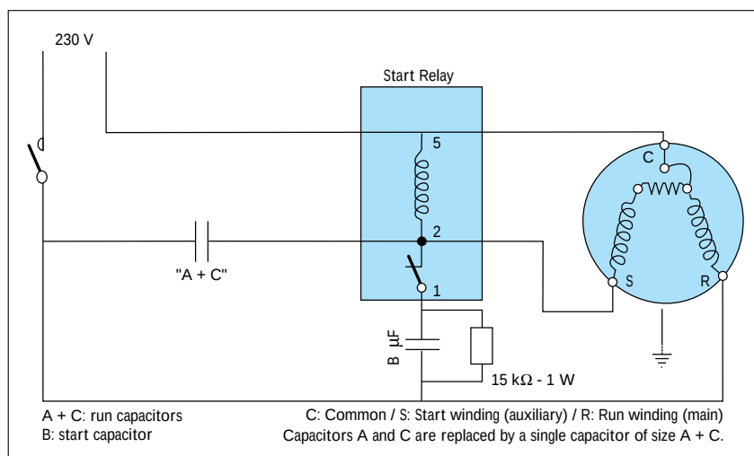
Single phase CSR wiring without trickle circuit
