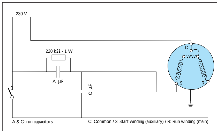
Single phase PSC wiring with trickle circuit
